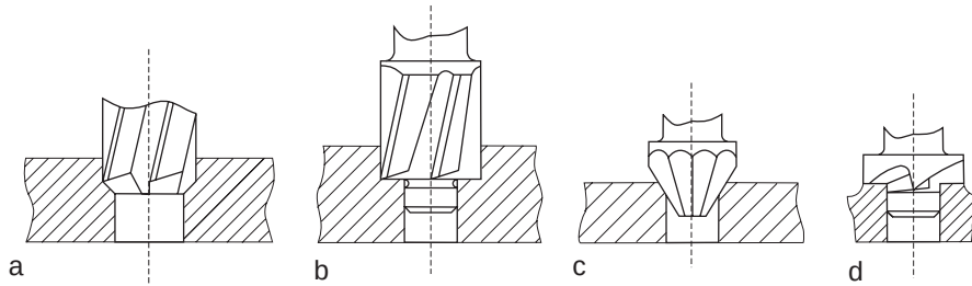
a, b, c, d - core drill different shapes (different surfaces) according to hole (surface) shape;
